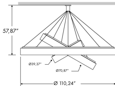
CEILING MOUNTED
