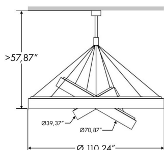
SUSPENDED
