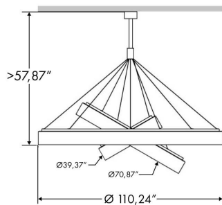
SUSPENDED
